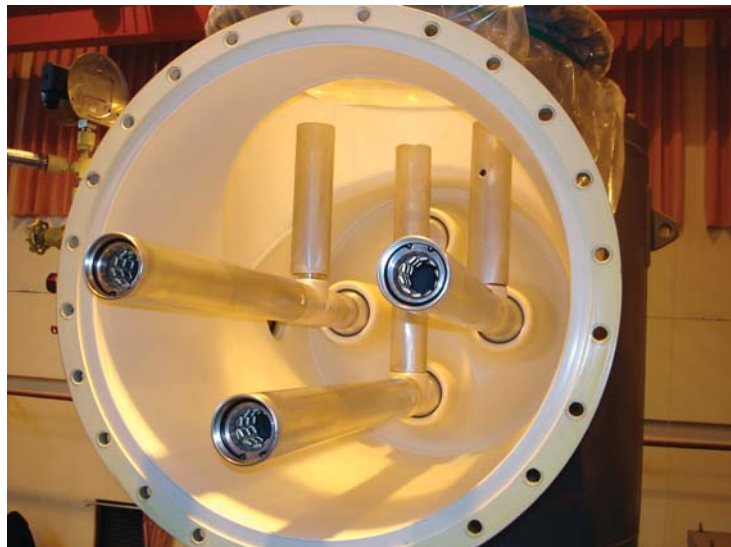
161KV 母線轉接氣室 Bus Bar Transition in Gas Compartment
